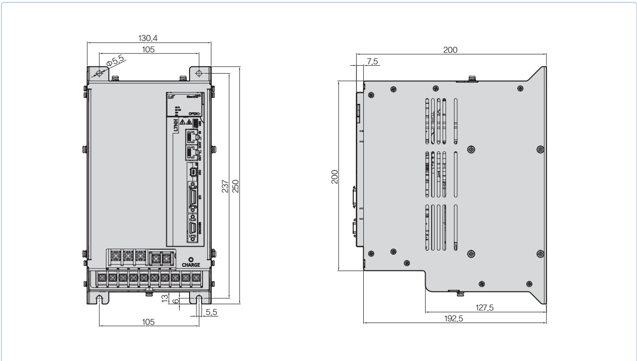
XDL-L7NB050U [Weight : 5.5kg (Fan-Cooling included)]
