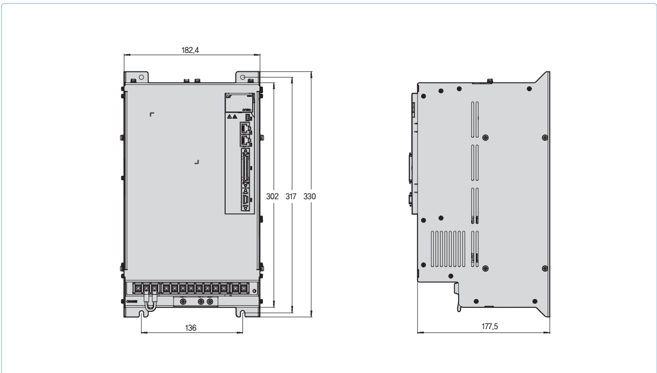
XDL-L7SA075 [Weight : 8.5kg(Fan-Cooling included)]
