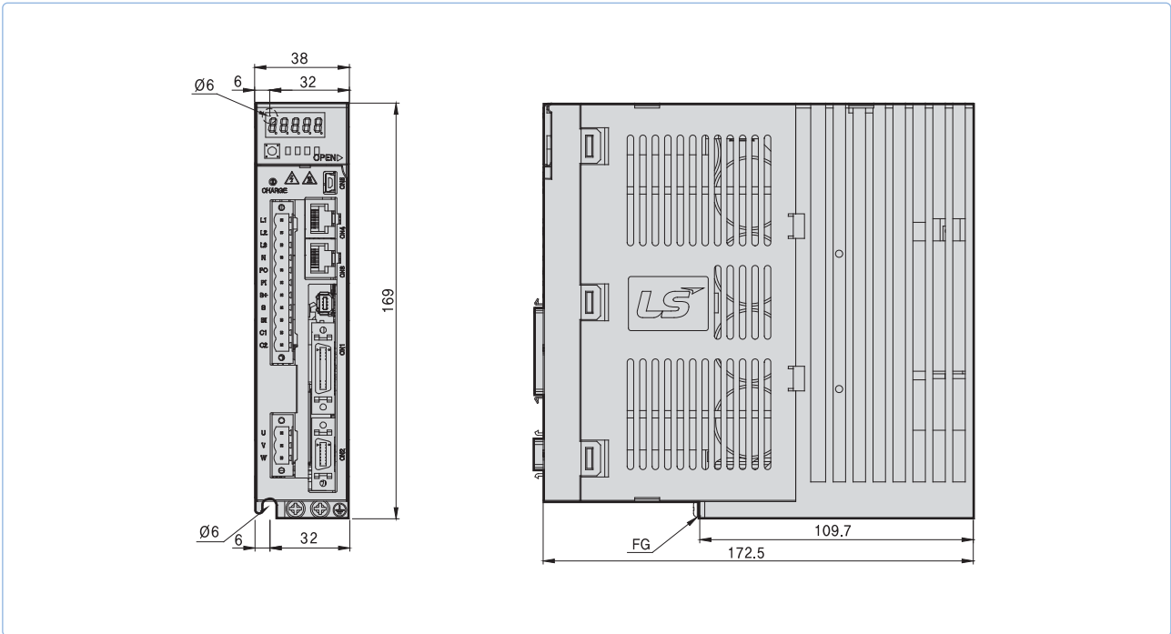
XDL-L7NA001B ~ XDL-L7NA004B[Weight : 1.2kg]
