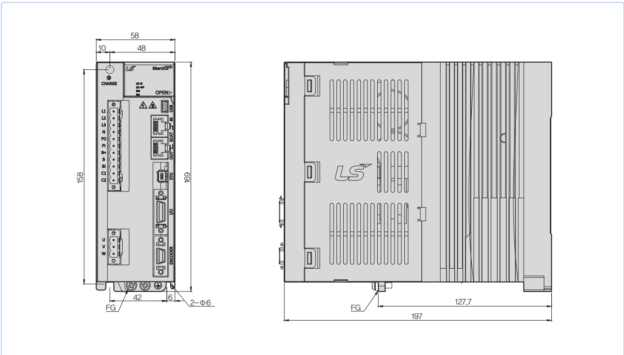
XDL-L7NHA008U / XDL-L7NHA010U [Weight : 1.5kg (Fan-Cooling included)]
