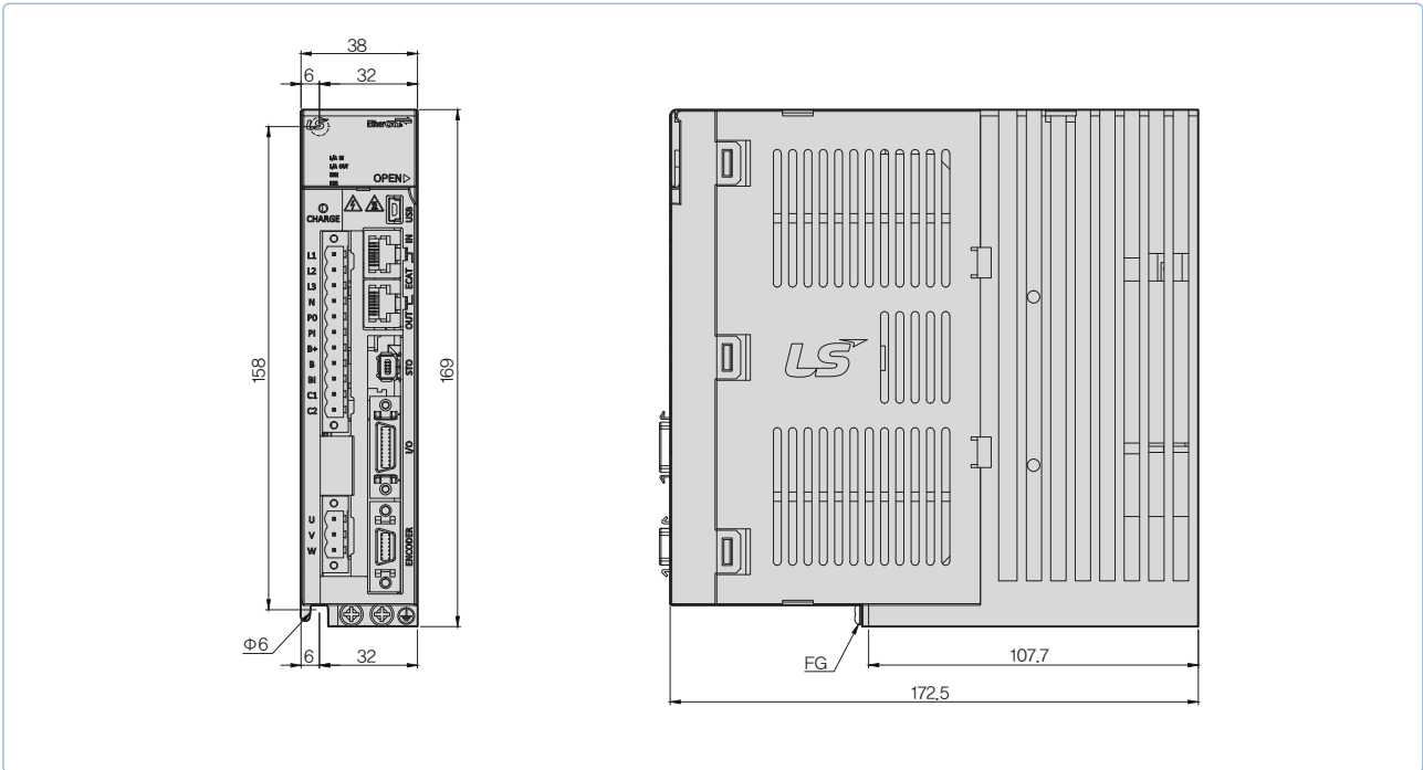
XDL-L7NHA001U ~ XDL-L7NHA004U [Weight : 1.0kg]
