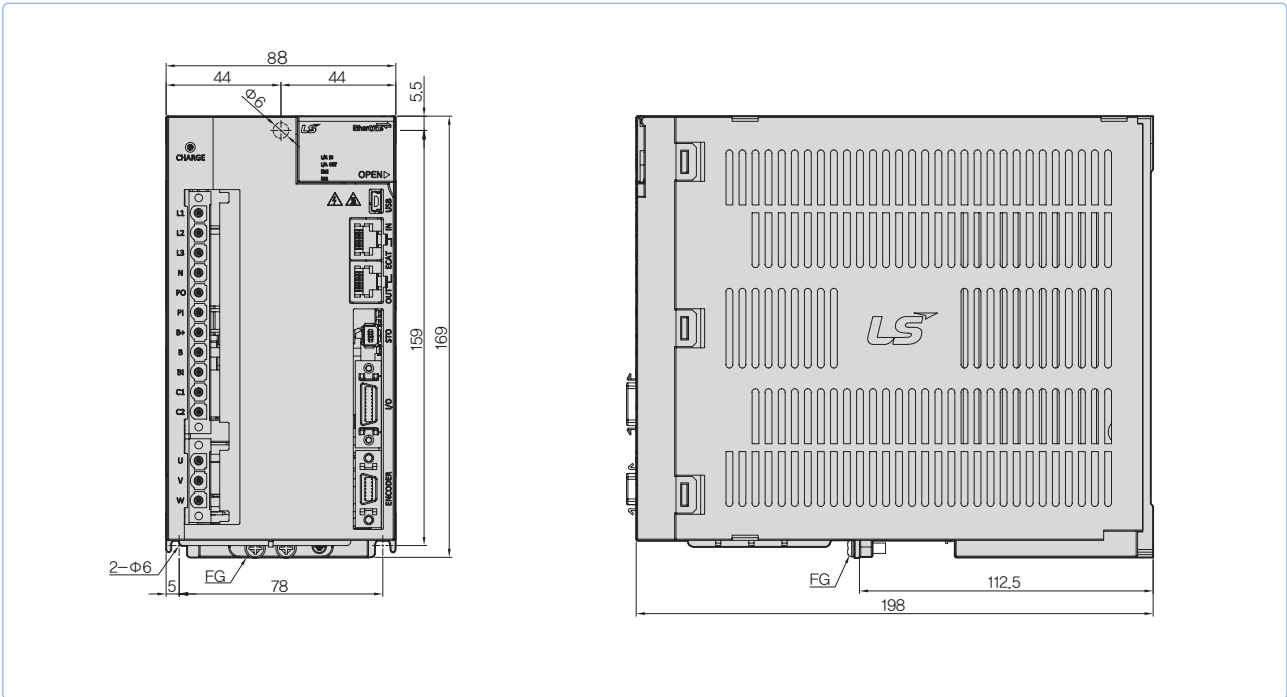
XDL-L7NHB020U / XDL-L7NHB035U [Weight : 2.5kg (Fan-Cooling included)]
