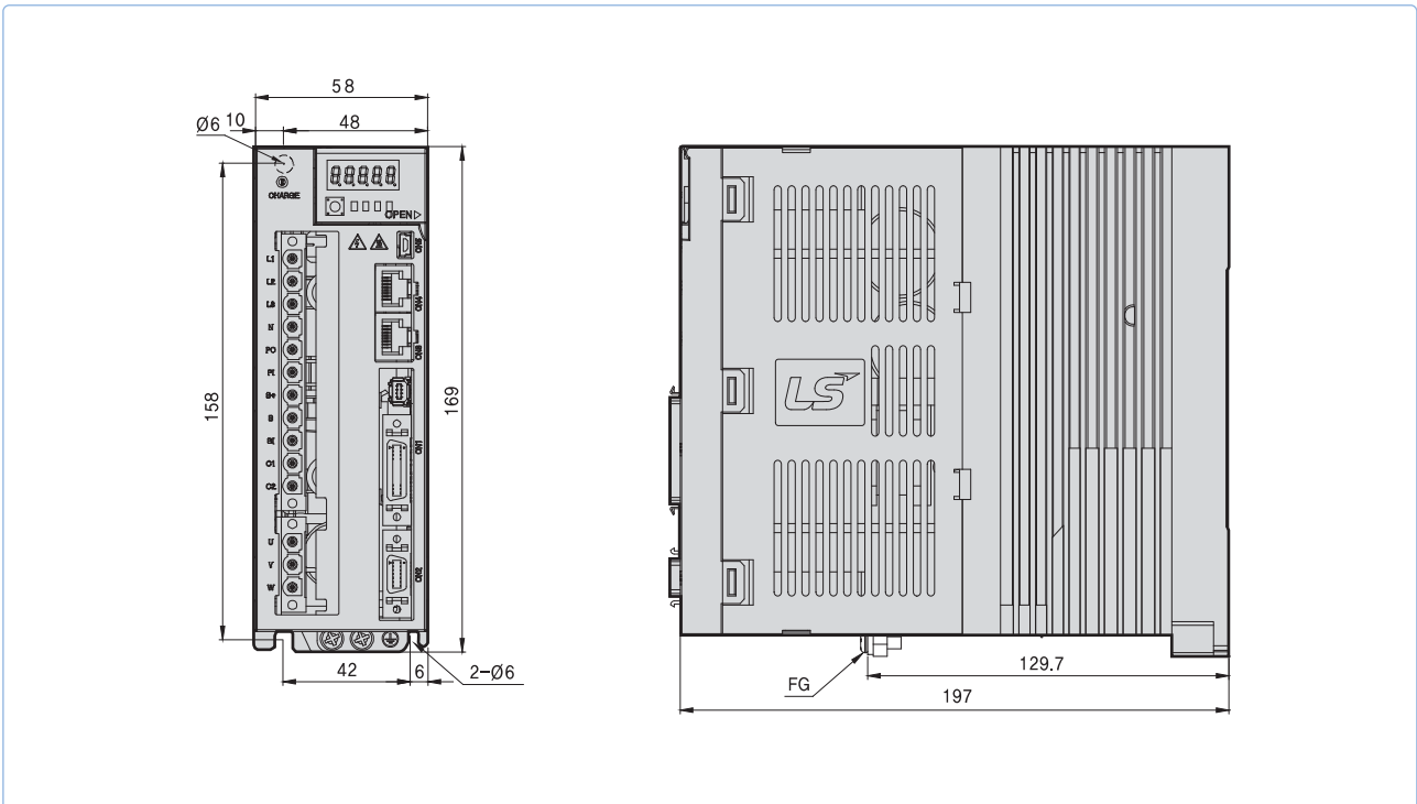
XDL-L7NA008B / XDL-L7NA010B[Weight : 1.5kg(Fan-Cooling included)]
