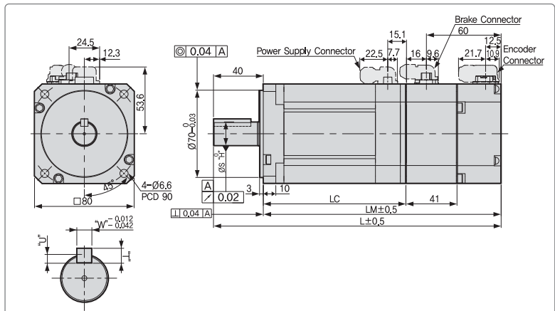
(Cross section of shaft key S/C 2:1)
