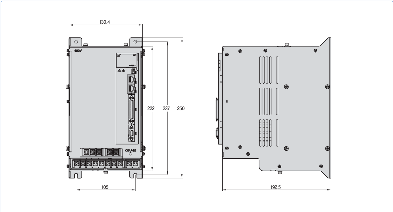
XDL-L7SB050 [Weight : 5.5kg(Fan-Cooling included)]
