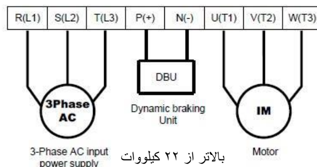
F3~F6 Power Terminal
